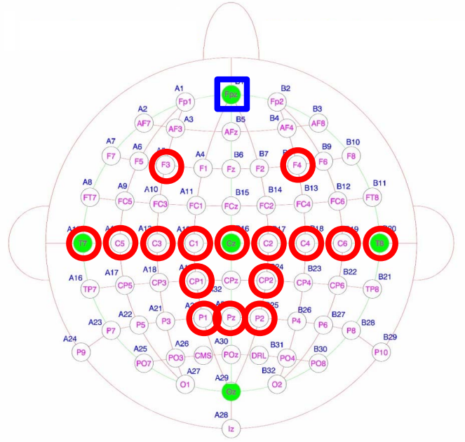
Fig. 6. The 10/10 system locations of EEG electrodes on a scalp. The graph is based on BIOSEMI’s 64-channels EEG cap layout. The red circles represent recoding electrodes chosen for experiments reported in this paper. The blue square is a ground electrode. A reference was attached to the left earlobe.
