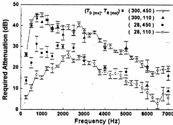
Figure 4: Subjective test results on the ERLR_f for different reverberation times in the echo-path model room.
