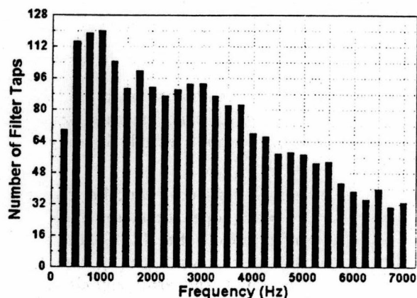
Figure 6: Desired SBEC filter tap profile.
