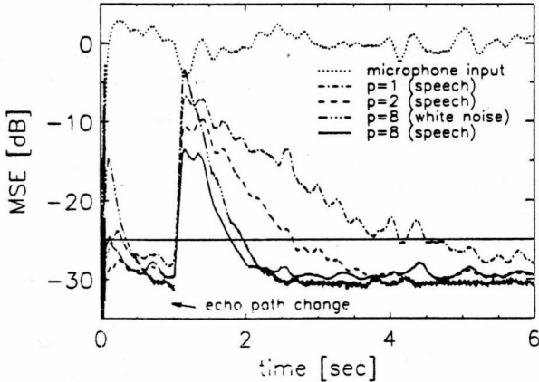
Fig. 6. Convergence curves for various projection orders.
