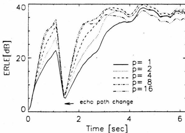
Fig. 4. Convergence curves for various projection order in the proposed subband echo canceller. The convergence speed of p=8 is almost the same as that of p=16 . (computer simulation)
