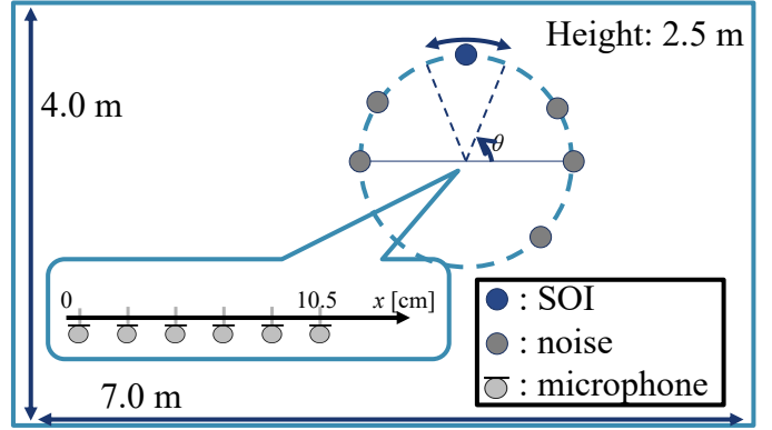
Fig. 1: Experimental sound source and microphone layout
