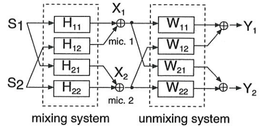
Fig. 1. BSS system configuration.
