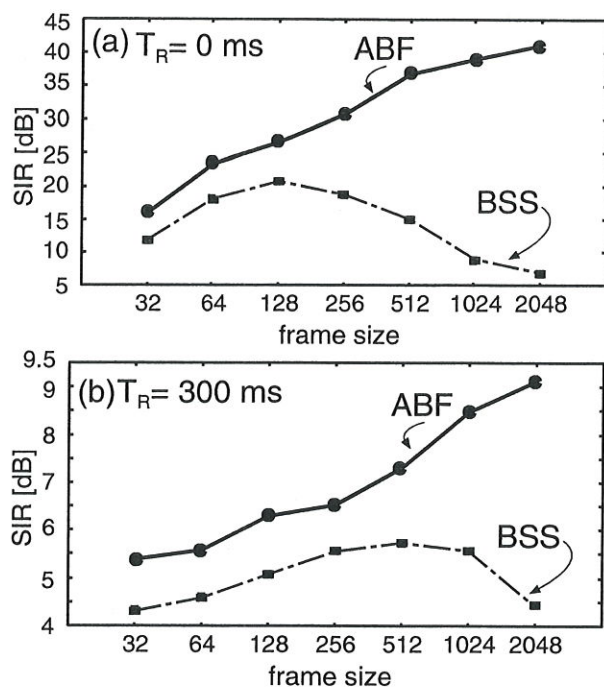
Fig. 4. Results of SIR for different frame sizes. The solid lines are for ABF and the dash-dotted lines are for BSS. (a) Non-reverberant test, (b) reverberant test ( T_R=300 ms).
