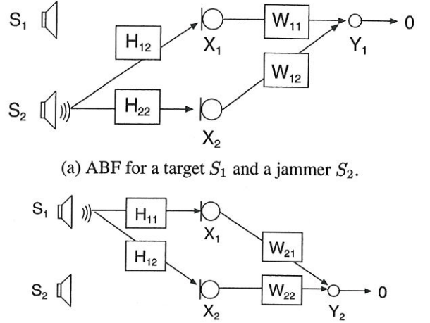
Fig. 2. Two sets of ABF-system configurations.
